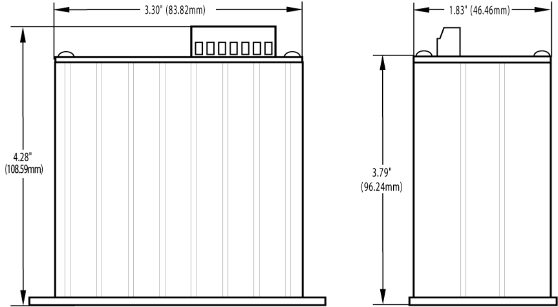
SNAP-PAC-SB1 and SNAP-PAC-SB2 Serial Brains
