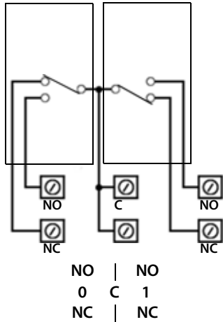
Terminals 0 and 1
