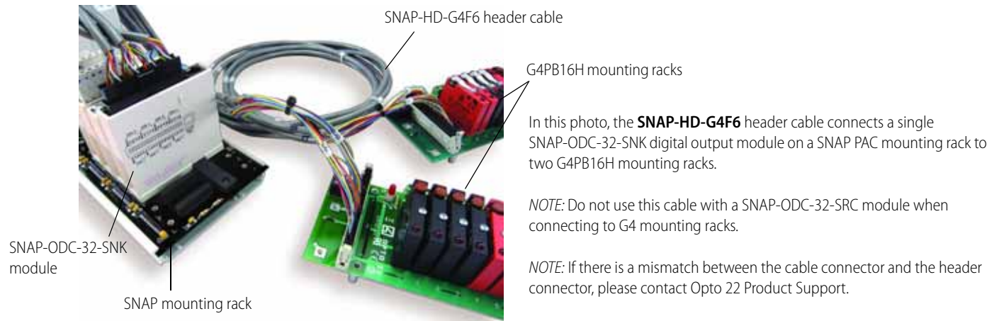
SNAP-HD-G4F6 cable
